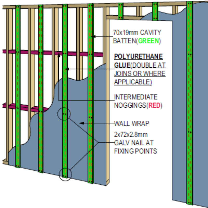
INTERMEDIATE NOGGINGS AND CAVITY BATTENS (WALL WRAP SHOWN)
